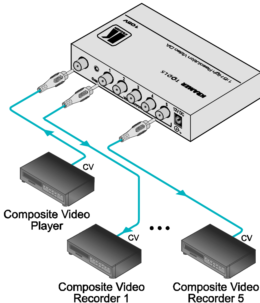
Figure 11: Connecting the 105V 1:5 High Resolution Video DA
