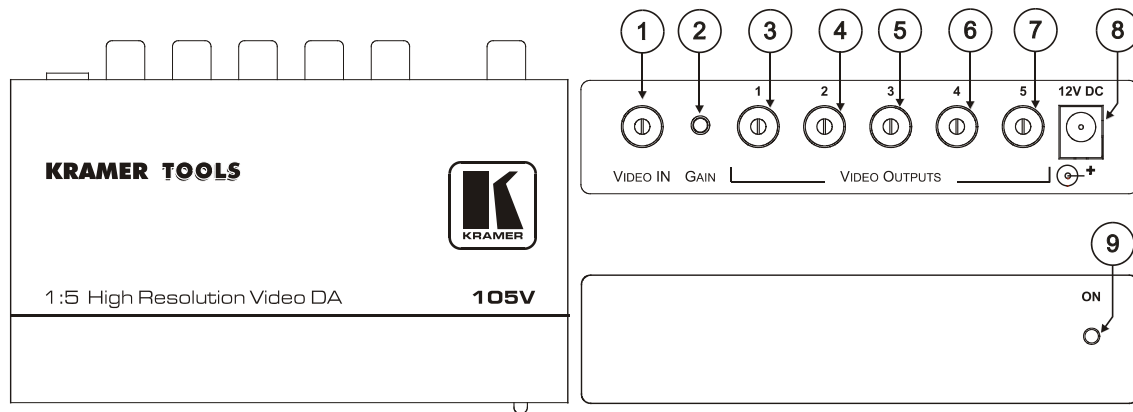
Figure 10: 105V 1:5 High Resolution Video DA
