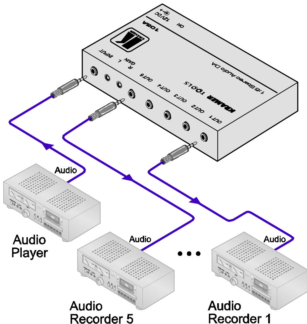
Figure 6: Connecting the 105A 1:5 Stereo Audio DA
