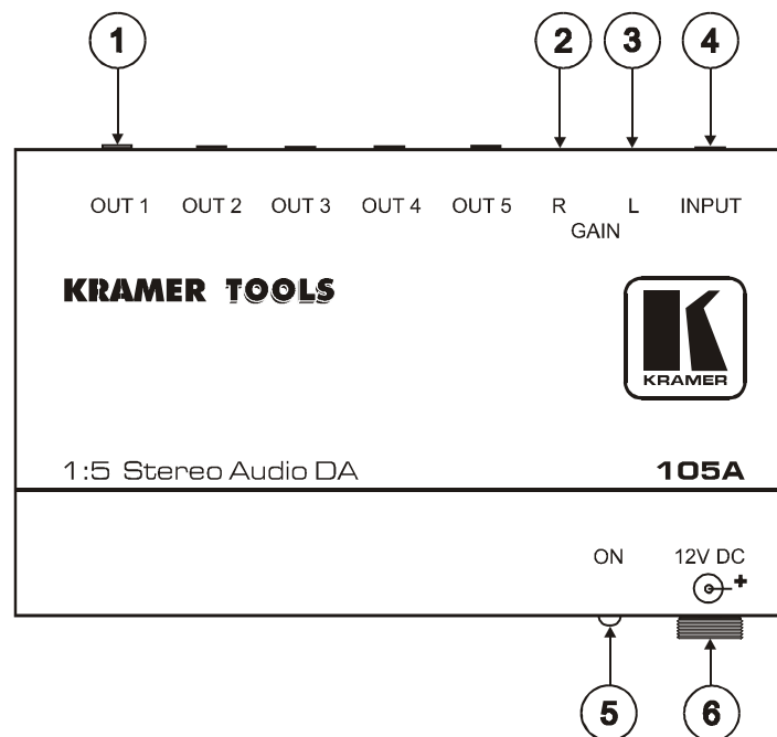
Figure 5: 105A 1:5 Stereo Audio DA
