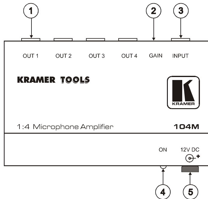
Figure 3: 104M Microphone Amplifier
