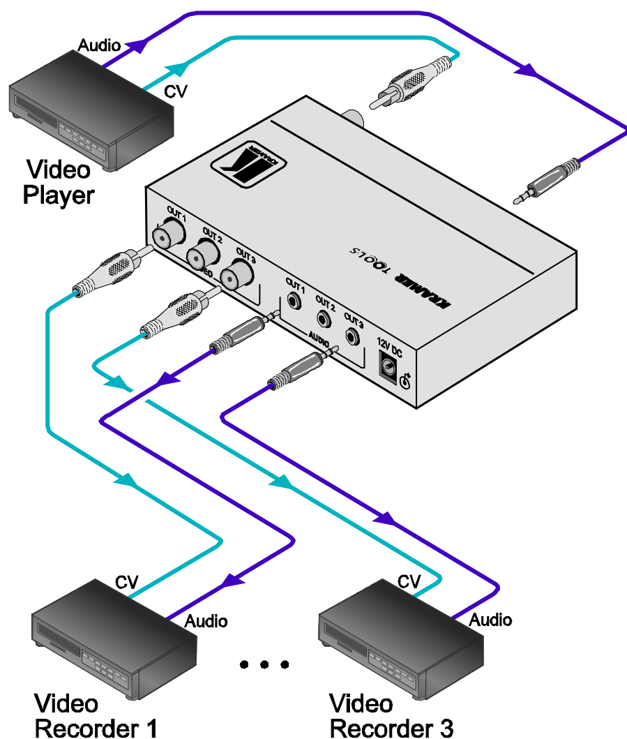
Figure 2: Connecting the 103AV 1:3 Audio-Stereo / Video DA
