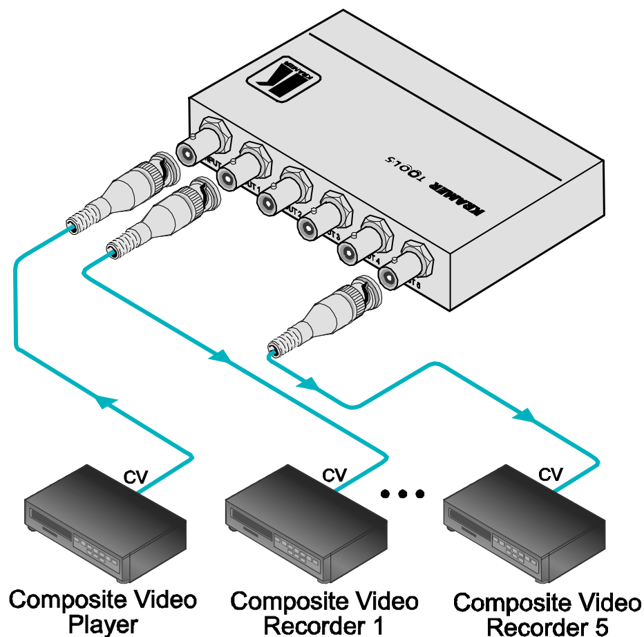
Figure 14: Connecting the 105VB 1:5 High Resolution Video DA
