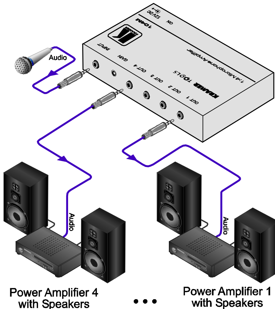
Figure 4: Connecting the 104M 1:4 Microphone Amplifier
