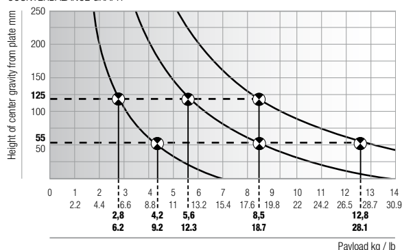
COUNTERBALANCE GRAPH
