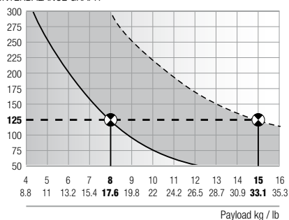
COUNTERBALANCE GRAPH
