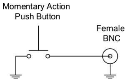
Figure: Contact Closure Style Trigger Button Circuit Diagram (SYNC)
