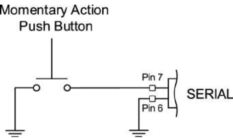
Figure: Contact Closure Style Trigger Button Circuit Diagram (SYNC)
